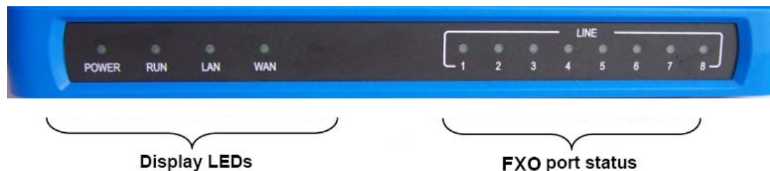
Figure 2: Diagram Of Unicorn 60x0 Display Panel
